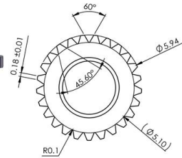
25T-6mm Output Shaft Spline
